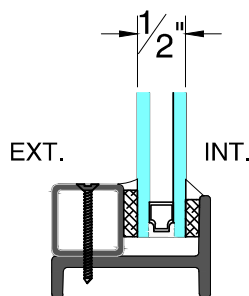
SQUARE STEEL GLAZING BEAD
