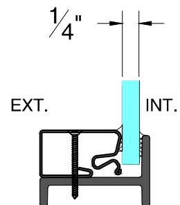
STEEL GLAZING BEAD
