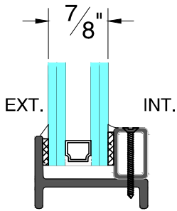
RECTANGULAR STEEL GLAZING BEAD
