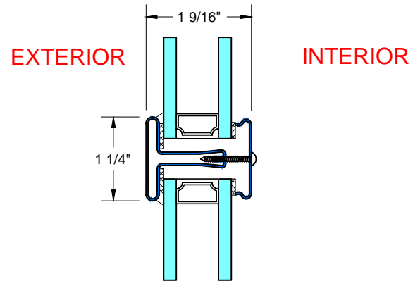
F TYPICAL HORIZONTAL MUNTIN
