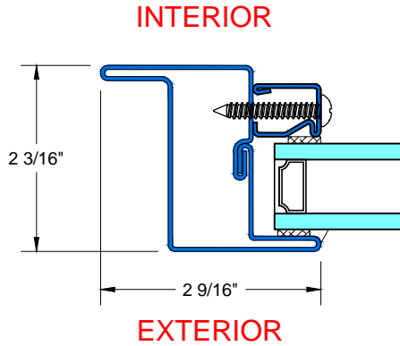
1 TYPICAL FIXED INTERIOR FLANGE
