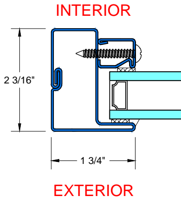
A TYPICAL LEFT JAMB
