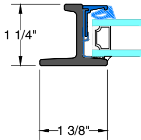
1 TYPICAL EXTERIOR FLANGE
