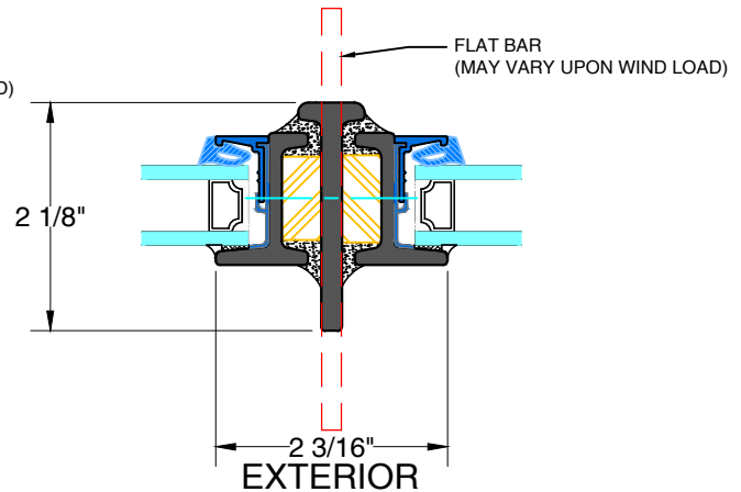
H TYPICAL JOINING MULLION
