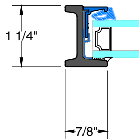
1 TYPICAL SHORT LEG FRAME
