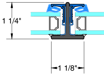
E TYPICAL VERTICAL MUNTIN
