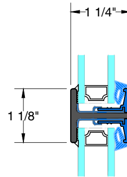
F TYPICAL HORIZONTAL MUNTIN
