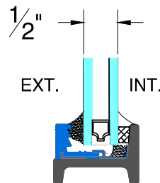
GB-13 GLAZING BEAD
