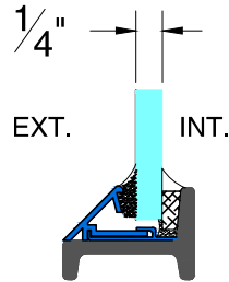
GB-15 GLAZING BEAD
