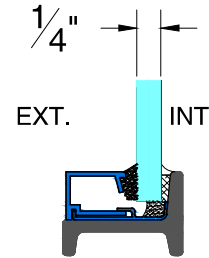
GB-06 GLAZING BEAD
