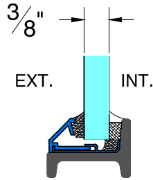
GB-04 GLAZING BEAD
