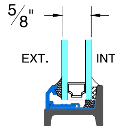
GB-12 GLAZING BEAD
