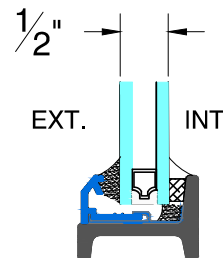
GB-12 GLAZING BEAD
