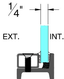
1/2" x 3/4" STEEL GLAZING BEAD
