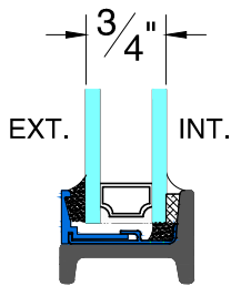
GB-05 GLAZING BEAD
