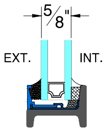
GB-05 GLAZING BEAD
