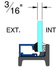
GB-06 GLAZING BEAD
