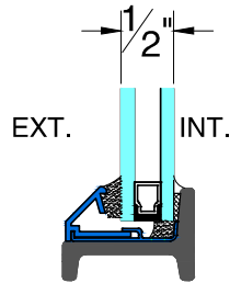
GB-04 GLAZING BEAD
