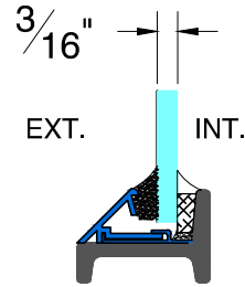
GB-15 GLAZING BEAD
