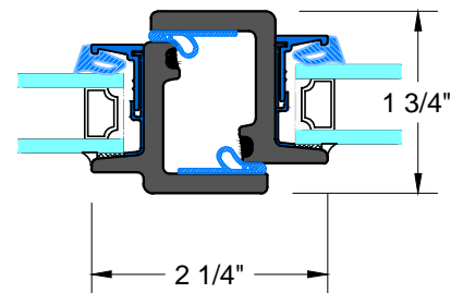
E TYPICAL FRENCH MEETING RAIL
