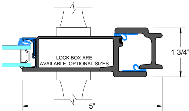
D TYPICAL SINGLE LOCKBOX
